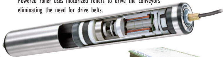
796 PRA Powered Roller Accumulator (rollers set low) Photo Eye Controlled 5 Week Shipment
