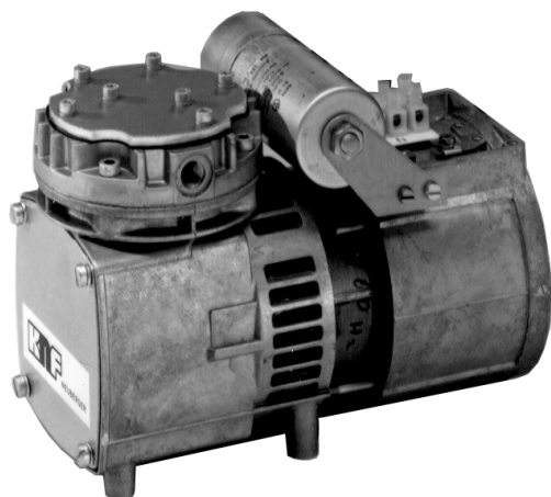
Figure 5: Diaphragm pump with an eccentric drive
