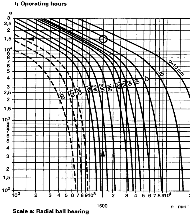
Figure 15: Lubrication limit t_f of radial ball bearings as a function of inner diameter d and rotational speed n . Source: Skf main catalogue 4000/IVT
