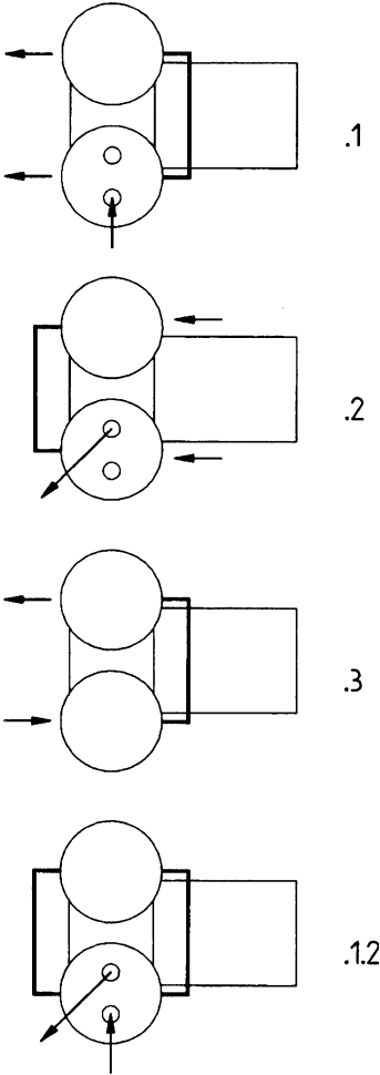
Figure 13: Types of connection of double-headed diaphragm pumps
