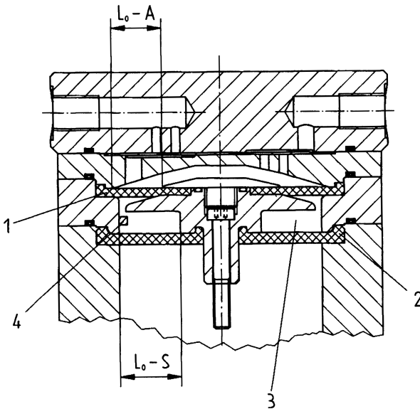
Figure 27: Basic construction of the diaphragm pump with a double diaphragm system
