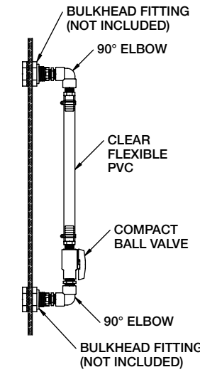
Single Valve Sight Gauge
