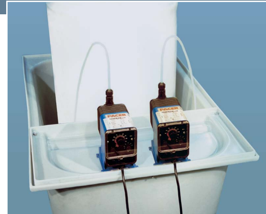
Polyethylene pump shelf supports most pumps and metering devices. Optional fiberglass shelves are available for pumps and metering devices totaling 25 pounds or more.
