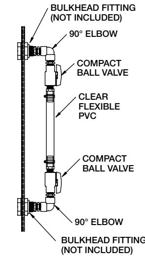
Double Valve Sight Gauge
