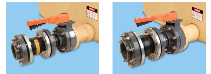
3" FDO (left) and 4" FDO (right) with flanged coupling, butterfly valve, and flexible expansion joint.
