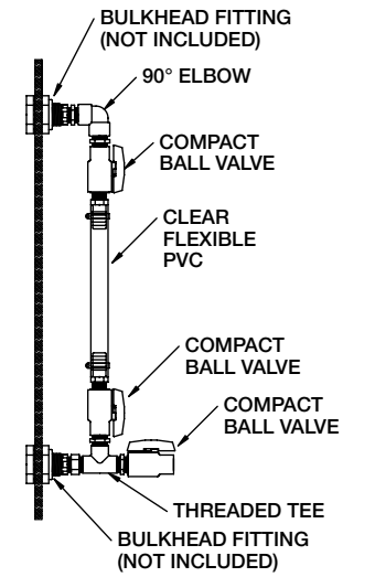
Triple Valve Sight Gauge
