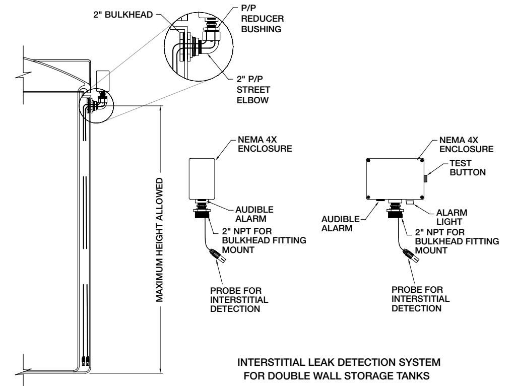
Interstitial Leak Detection System with Audible and Visual Alarms
