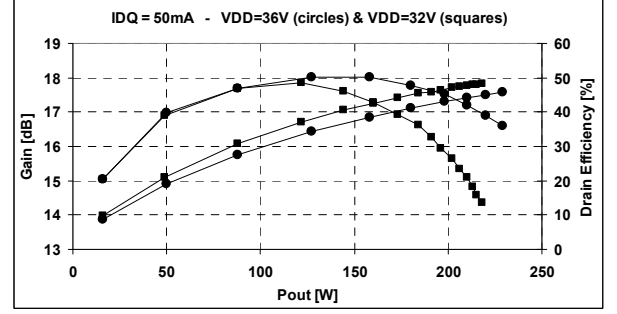
Fig. 9 Pulsed CW data at 1030MHz for gain and drain efficiency vs. output power for one LDMOS transistor biased at 50mA quiescent current at 32V and 36V.
