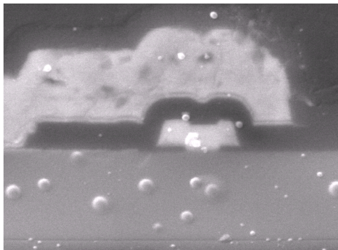
Figure 1. SEM cross-section of Integra's 0.5 \mu m GaN HEMT die with double field plate design.
