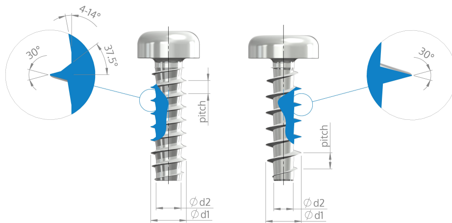
Left: STP thread geometry, Right: STPA Geometry
