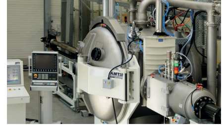
LPCS Spray Installation
