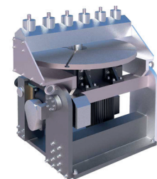
Multiple Stations
